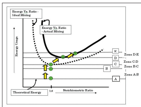
▲ Fig 2. Zones of lost energy.
