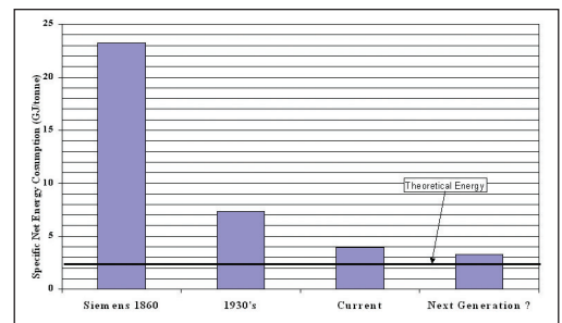
▲ Fig 1. Developments in energy efficiency: container furnace development.
